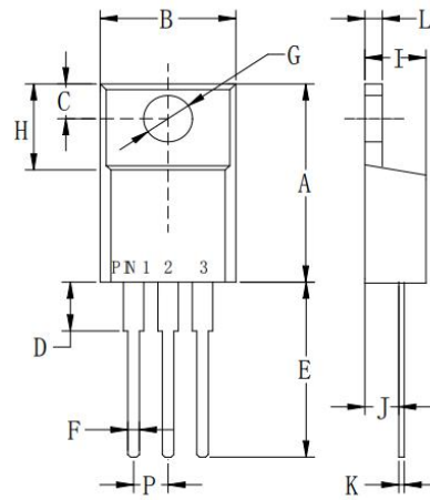
ITO-220AB(TBR30C150CTF)
