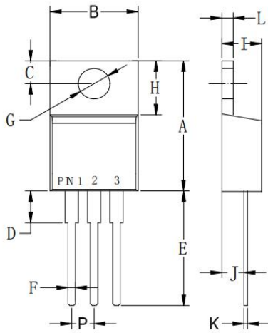
TO-220AB(TBR30C150CT)
