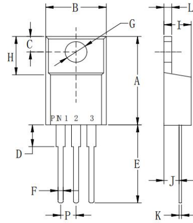
ITO-220AB(TBR10100CTF)
